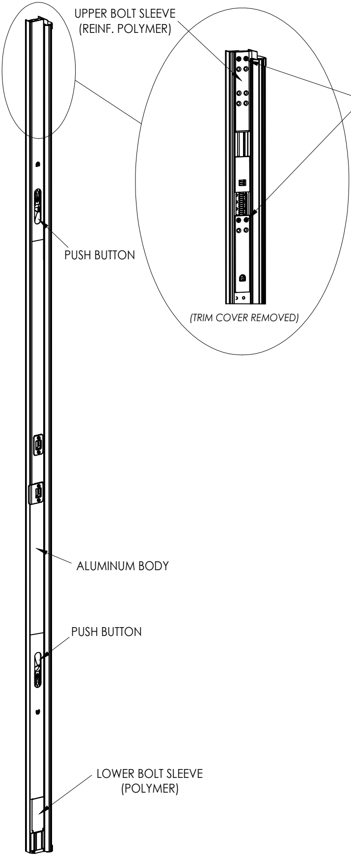
ULTIMATE PUSH BUTTON ASTRAGAL
