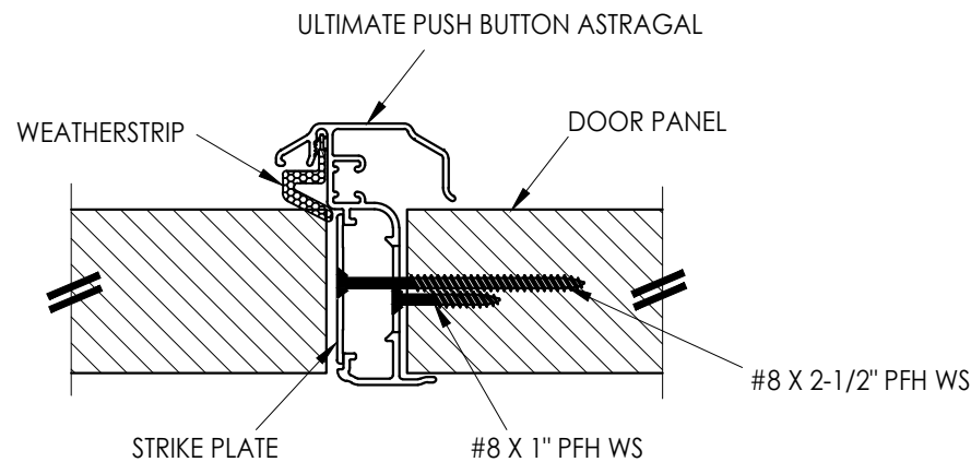
2/4 HORIZONTAL CROSS SECTION
